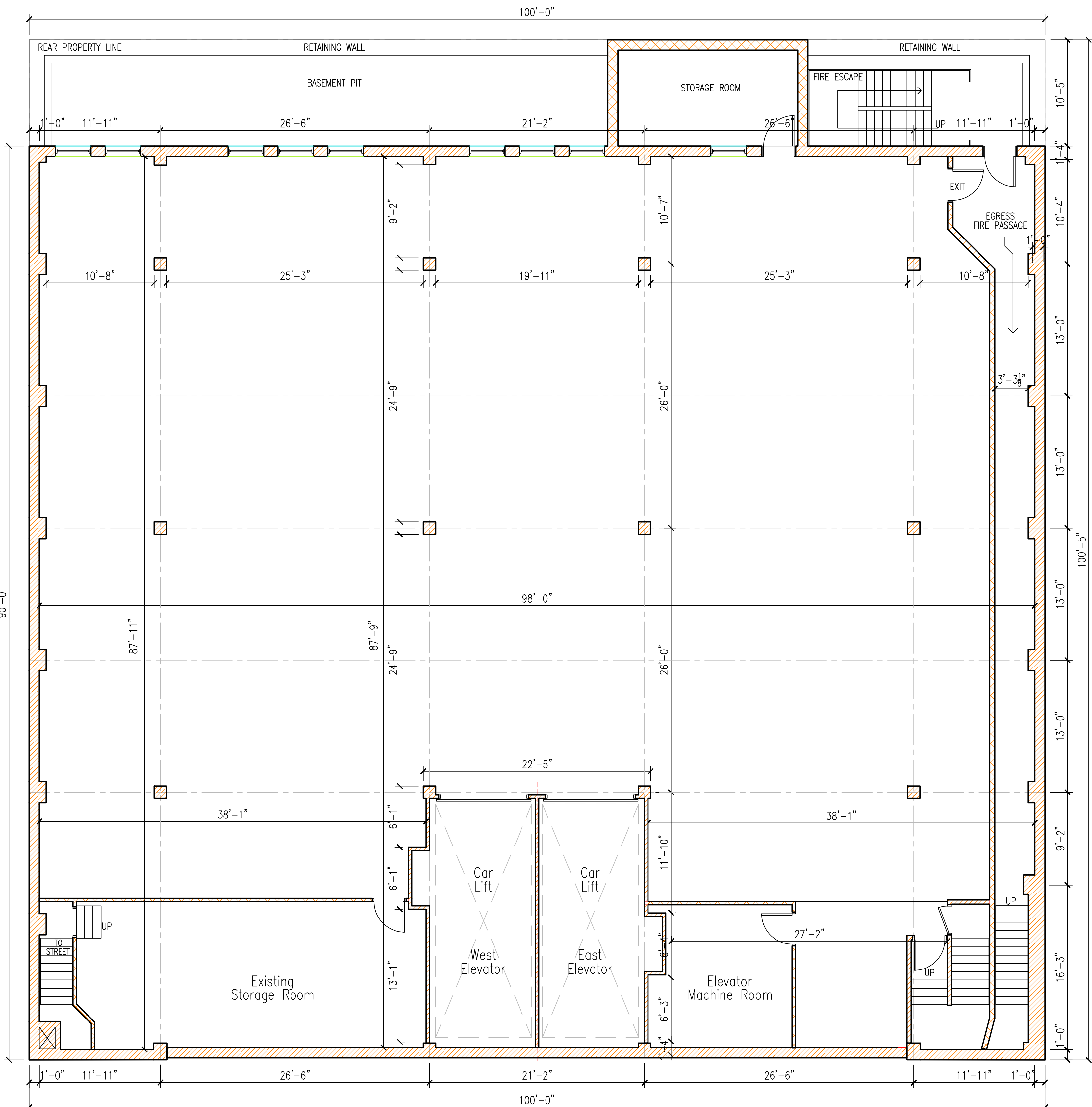
337 East 64th Street Basement Plan
