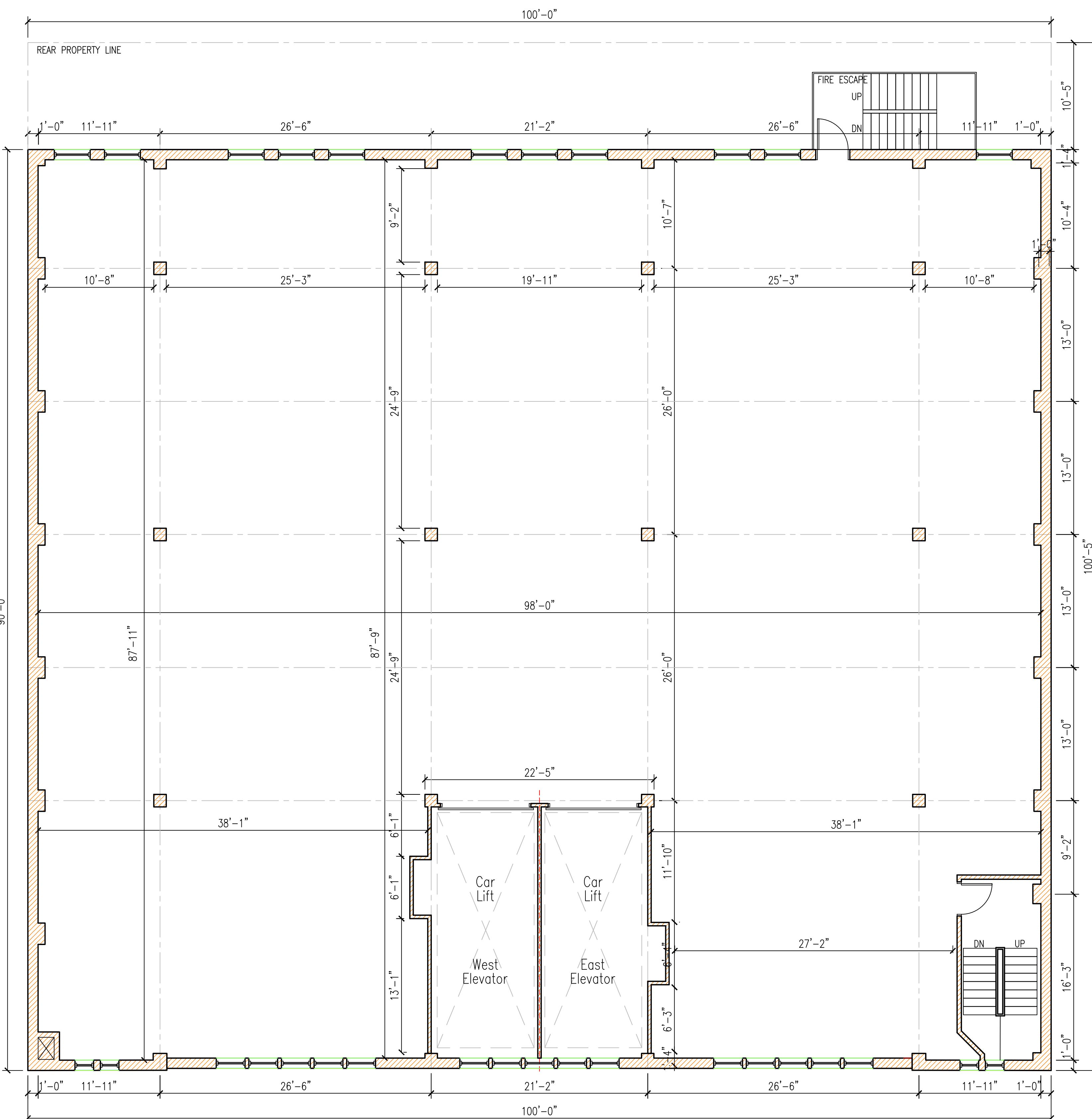
337 East 64th Street 2nd-3rd Floor Plan
