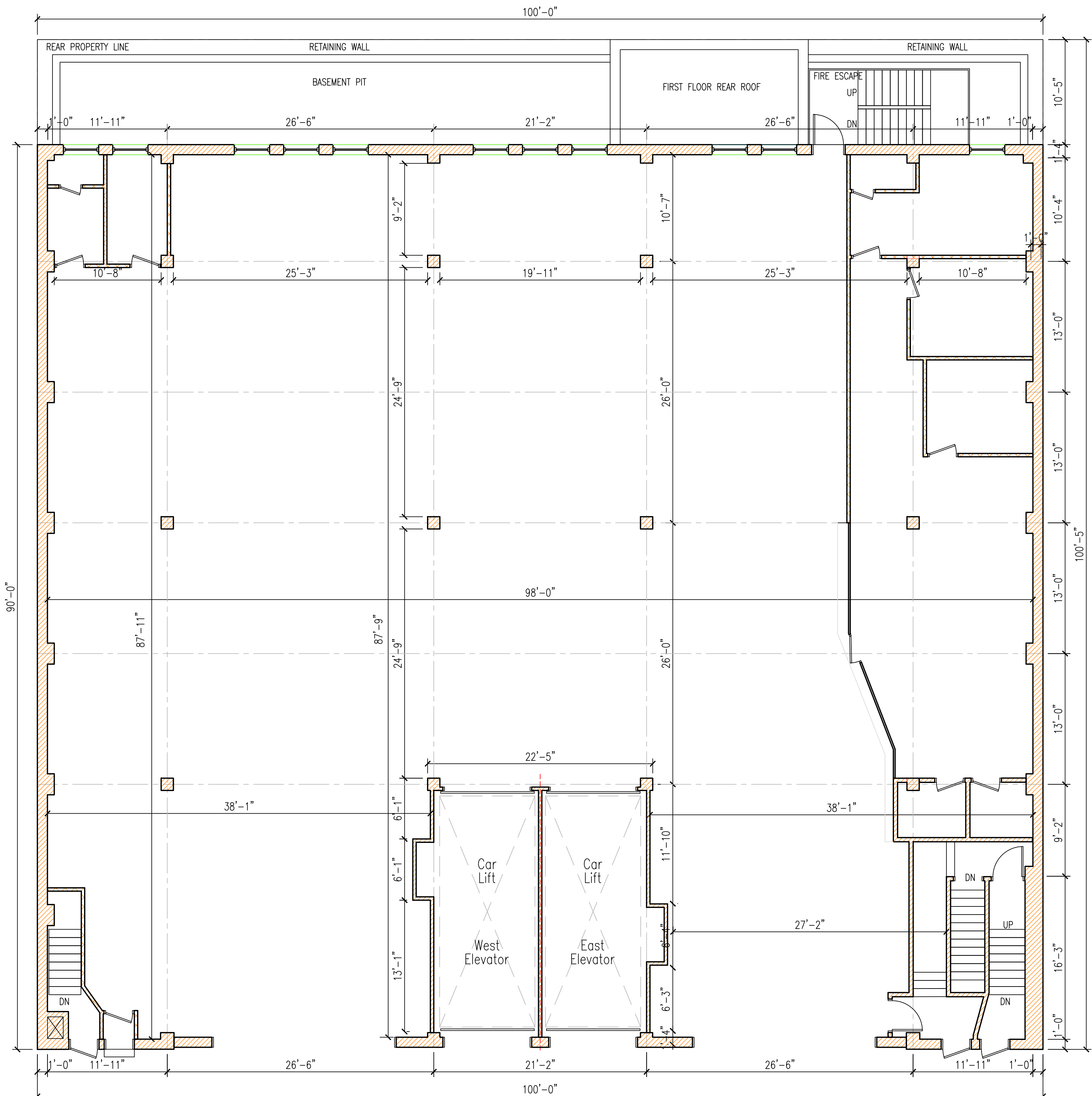
337 East 64th Street 1st Floor Plan
