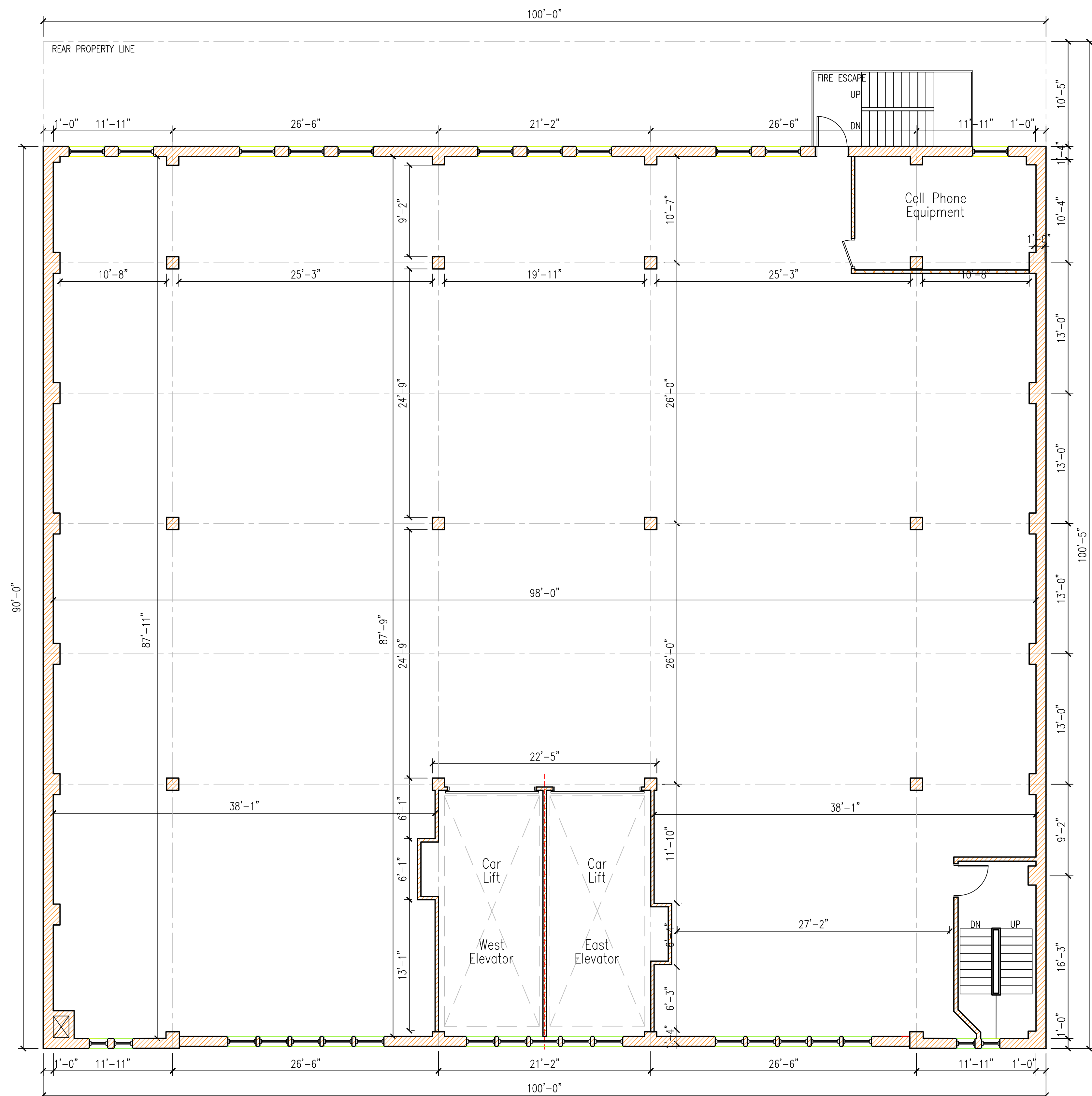
337 East 64th Street 4th Floor Plan
